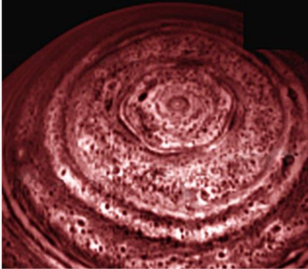
Polar Image of Saturn by Cassini
