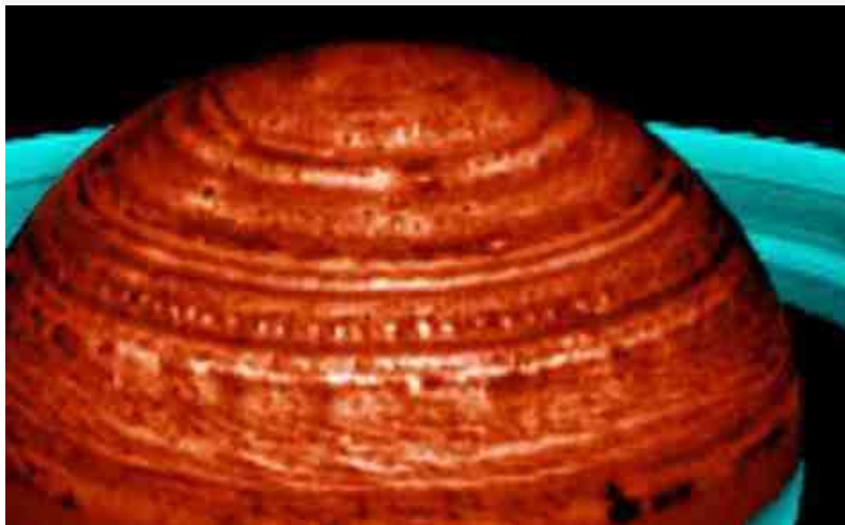
Polar Image of Saturn by Cassini
